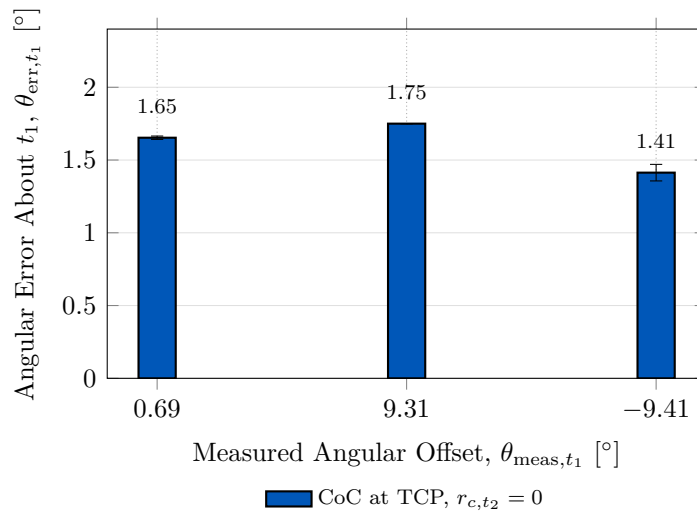
Figure 5.4: Angular error with the CoC at the TCP.
