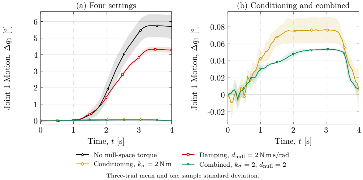
Figure 5.11: Joint motion during the virtual disturbance.
